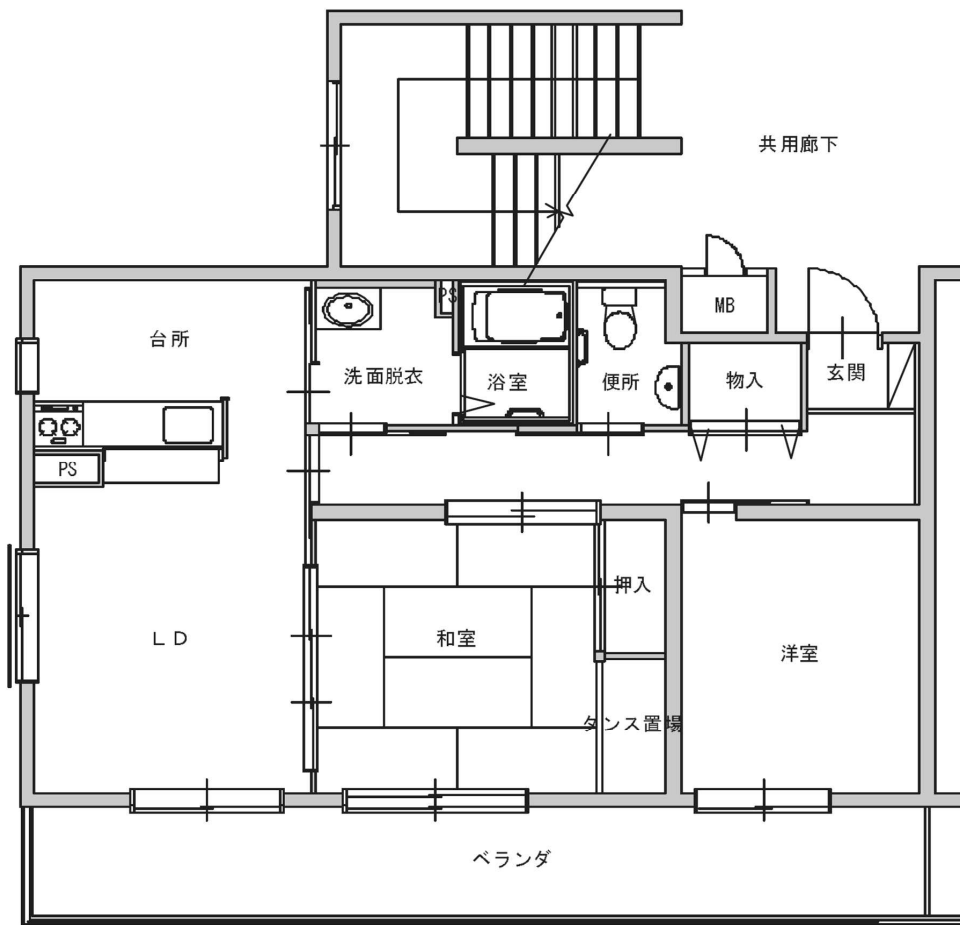
2LDKY (69.02m 2 )
