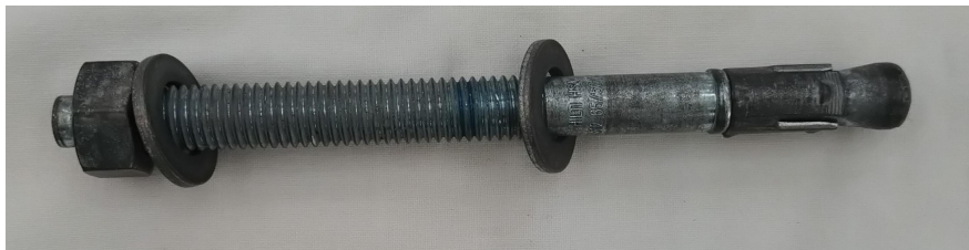
HILTI HSA M12×145 65/50/15
