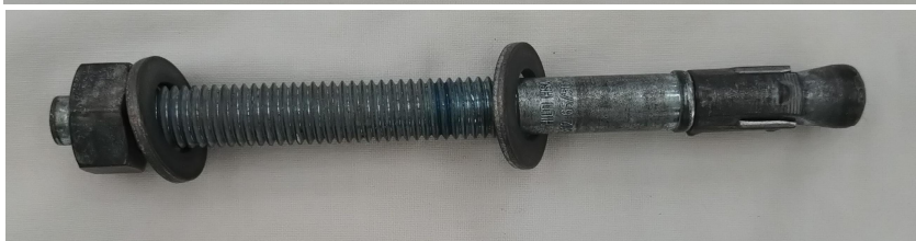
HILTI HSA M12×145 65/50/15
